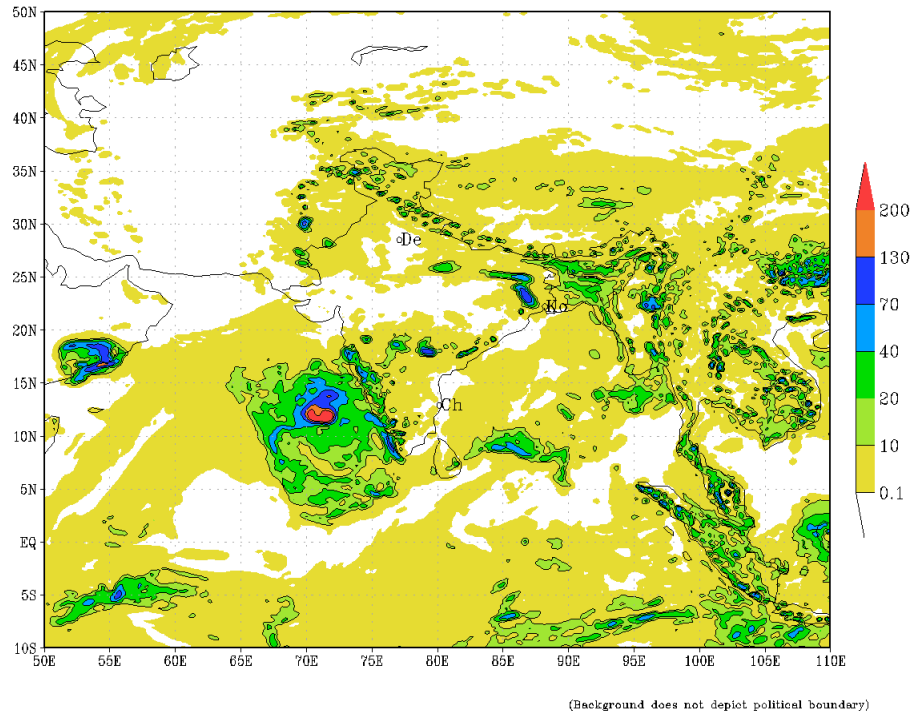
IMD :GFS MODEL(12 Km) RAINFALL (mm) FORECAST (24 HR) based on 00 UTC of 31-05-2020 valid for 03 UTC of 01-06-2020
